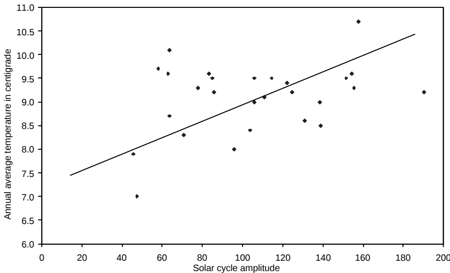
Figure 4: Solar Cycle Amplitude relative to Temperature 1705 to 2000.
