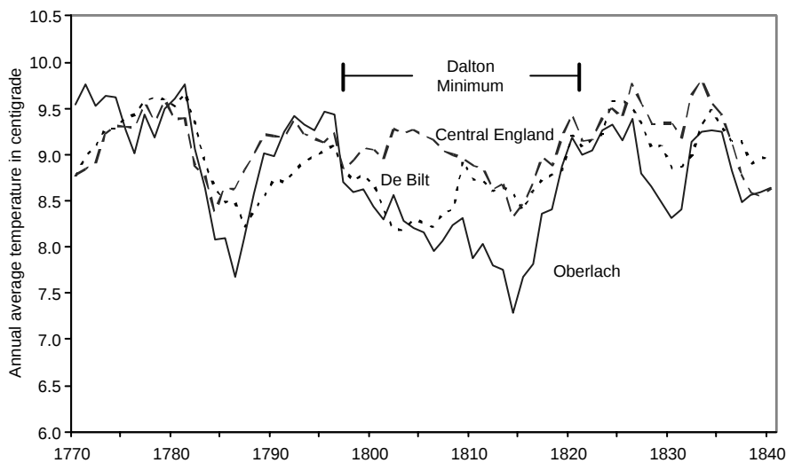
Figure 2: Annual Average Temperatures for Three European Stations 1770–1840.
