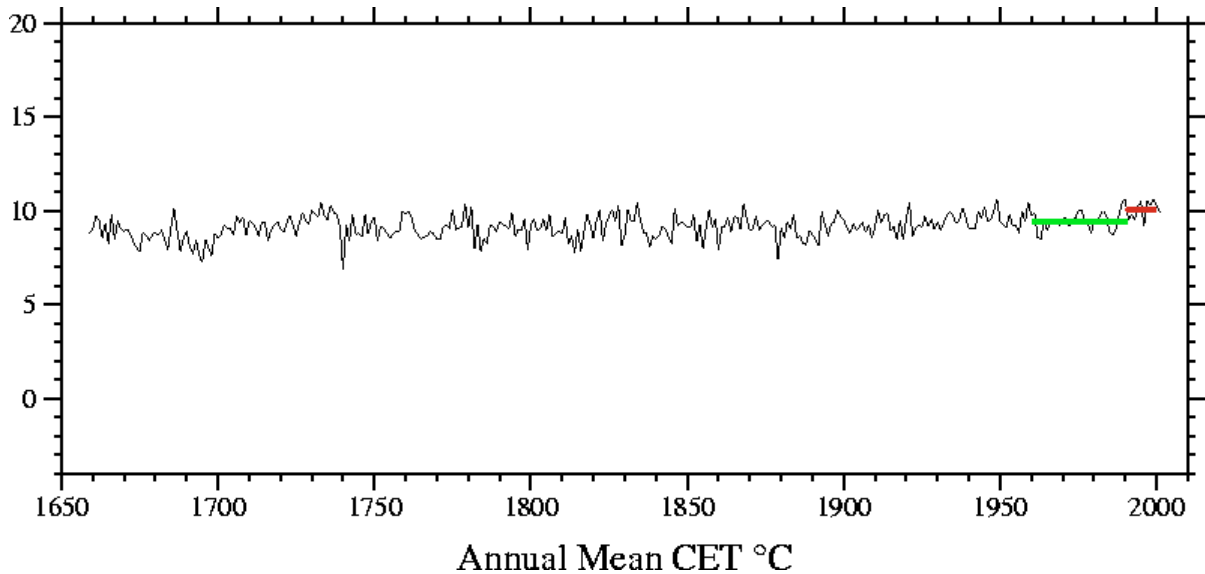
Figure 8. Temperature record for Central England since 1650
