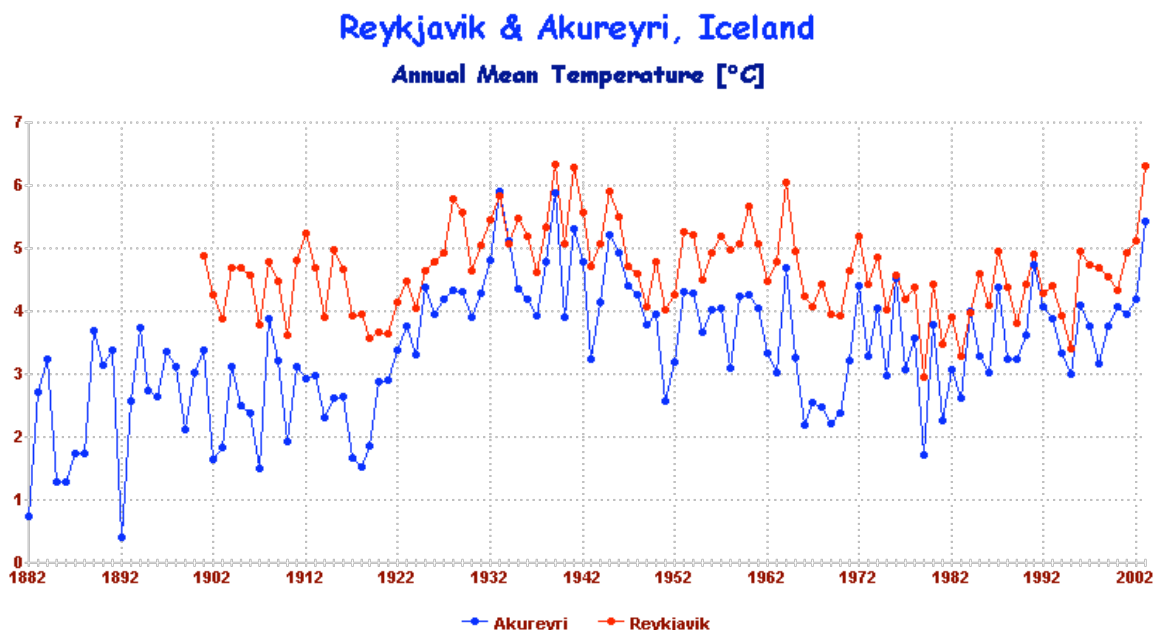
Figure 9. Temperature records for Reykjavik and Akureyri, Iceland
