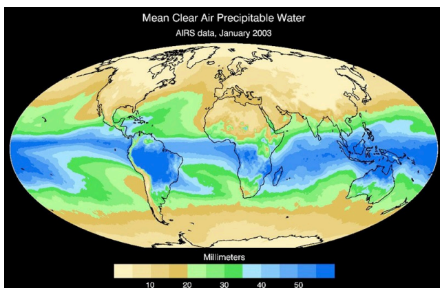
Figure 16. Total water vapour in the atmosphere for the month of January 2003, measured in mm. High value over 50mm, low to zero. (Encyclopaedia of Earth 2008)
