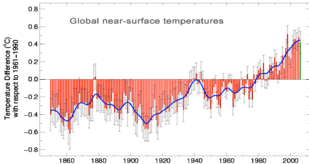
Figure 1. Mean Annual Global Surface Temperature Anomaly (Brohan et al 2006) showing 95% confidence levels
