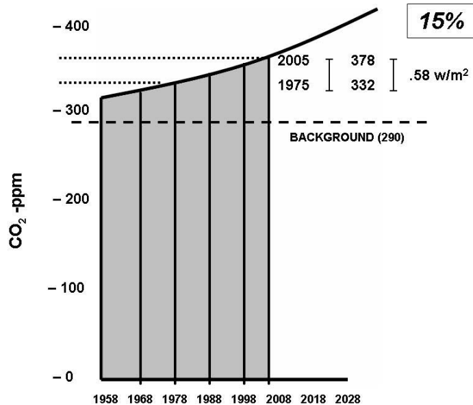
Figure 9. Illustration of relative comparison of water-vapor cirrus cloud and CO 2 suppression of outgoing longwave radiation (OLR). Global circulation models (GCMs) assume that more rainfall due to CO 2 doubling inhibits OLR (positive feedback) and that this causes additional warming. Observational analysis of enhanced global rainfall however, indicates a weak negative water-vapor cirrus feedback loop and therefore little global warming.
