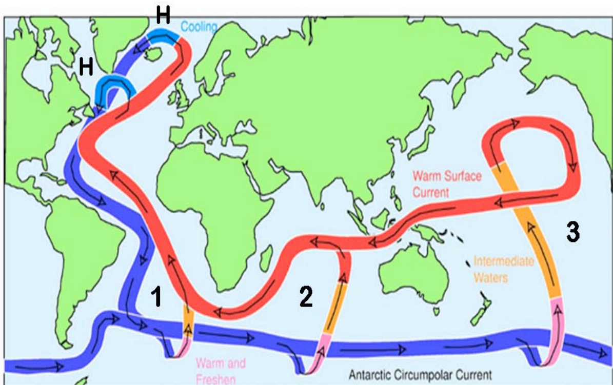
Figure 5. Idealized new estimate of the deep water Global Ocean Conveyor Belt showing the typical locations in the Southern Hemisphere of the required return cold upwelling circulation (areas 1, 2, 3) to balance the North Atlantic thermohaline ocean subsidence (H areas). Figure courtesy of John Marshall, of MIT.
