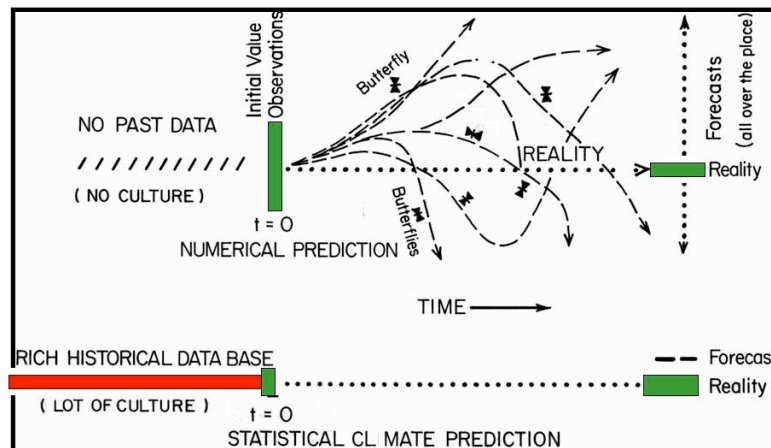
Figure 16. Illustrating the two types of climate prediction. The top diagram gives a depiction of initial value numerical modeling where prior data is not consulted and after 10-15 days the non-linear imperfections of the model grows into random turbulence (or butterflies). The bottom diagram shows statistical prediction which is based on how the atmosphere-ocean functions in many seasons or many years of past data.
