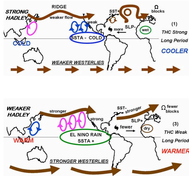
Figure 6. Comparison of typical global wind patterns when the Atlantic Thermohaline Circulation (THC) has been strong for a long period and cold water upwelling in the Southern Hemisphere has been strong. Global temperatures become cooler than average (top). Bottom diagram shows the typical global wind patterns when the Atlantic THC has been weak for a long period and there has been reduced cold water upwelling in the Southern Hemisphere. The globe becomes warmer during these periods.
