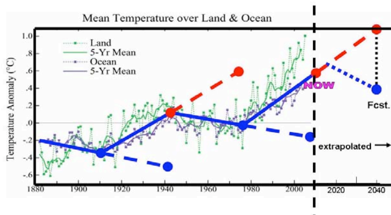
Figure 4. Same as Figure 3, but showing how much error one would have by extrapolating a cooling or warming curve beyond 30-35 years. The current 1975-2005 warming curve should not be expected to continue. It is likely that a global cooling trend will set in within the next few years. My forecast global temperature for 2040 is below the value of today's global temperature.
