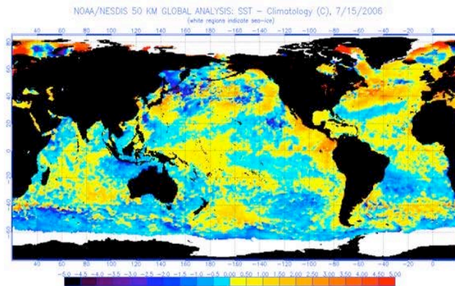
Figure 2. Example of the emerging El Niño for 2006.
