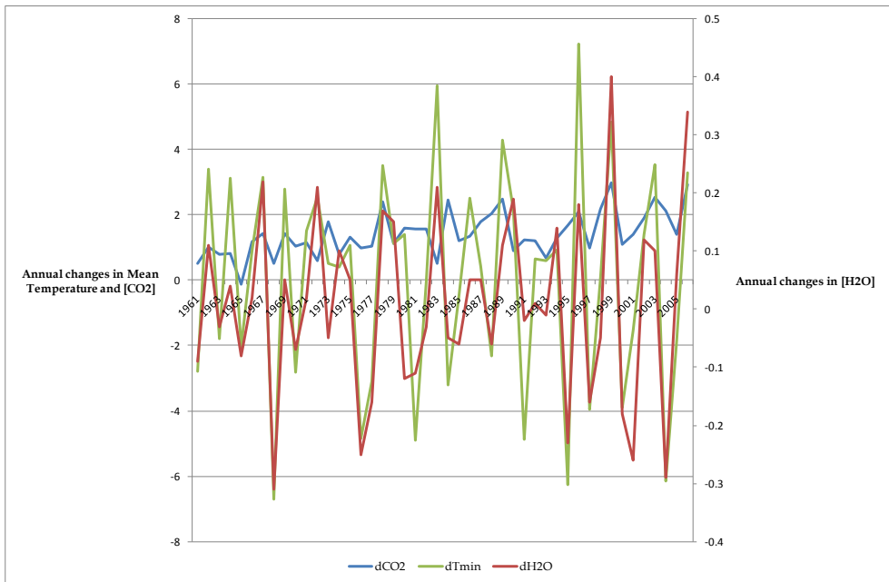
Fig.3 Annual changes in mean temperature, [CO_2] and [H_2O] , New York 1960-2006
