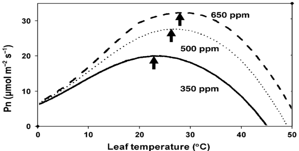
Fig. 4 The response of light-saturated net photosynthesis (Pn) to changes in leaf temperature at different atmospheric CO 2 concentrations.
